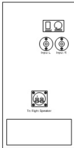
Left Speaker from behind
